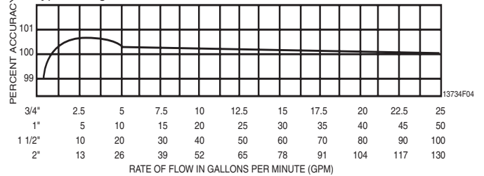
Typical Registration Curve
