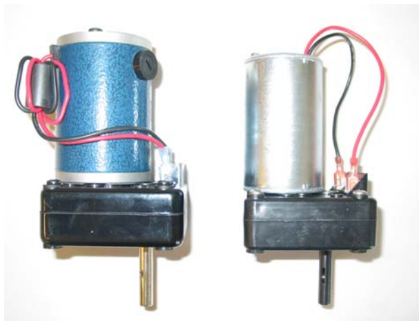
Figure 2. Old Pump Motor Gearbox
