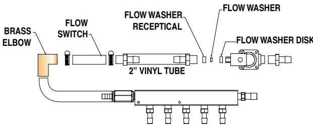
Summit E "Do it Yourself" Flush Manifold Assembly
