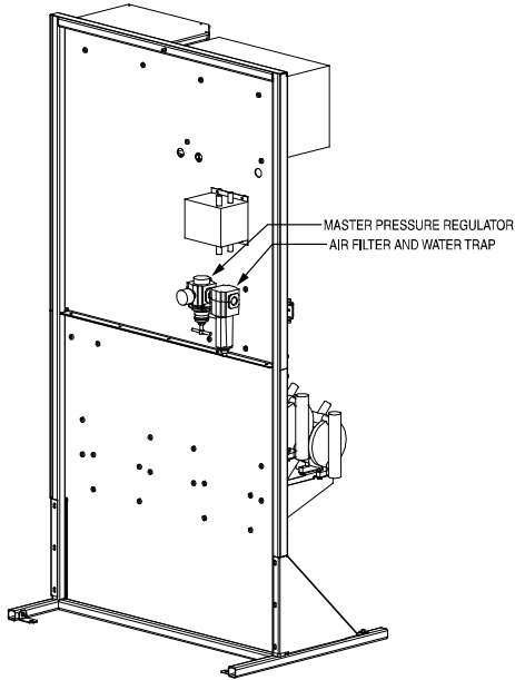
Grip V-B System, back side
