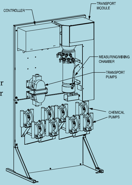
Grip V-B System, front side
