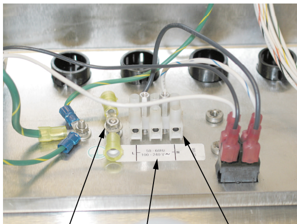
Ring Terminal Terminal Block Sticker Moved to Front of Terminal Block Taller Terminal Block Inside of Summit, TUV Compliant
